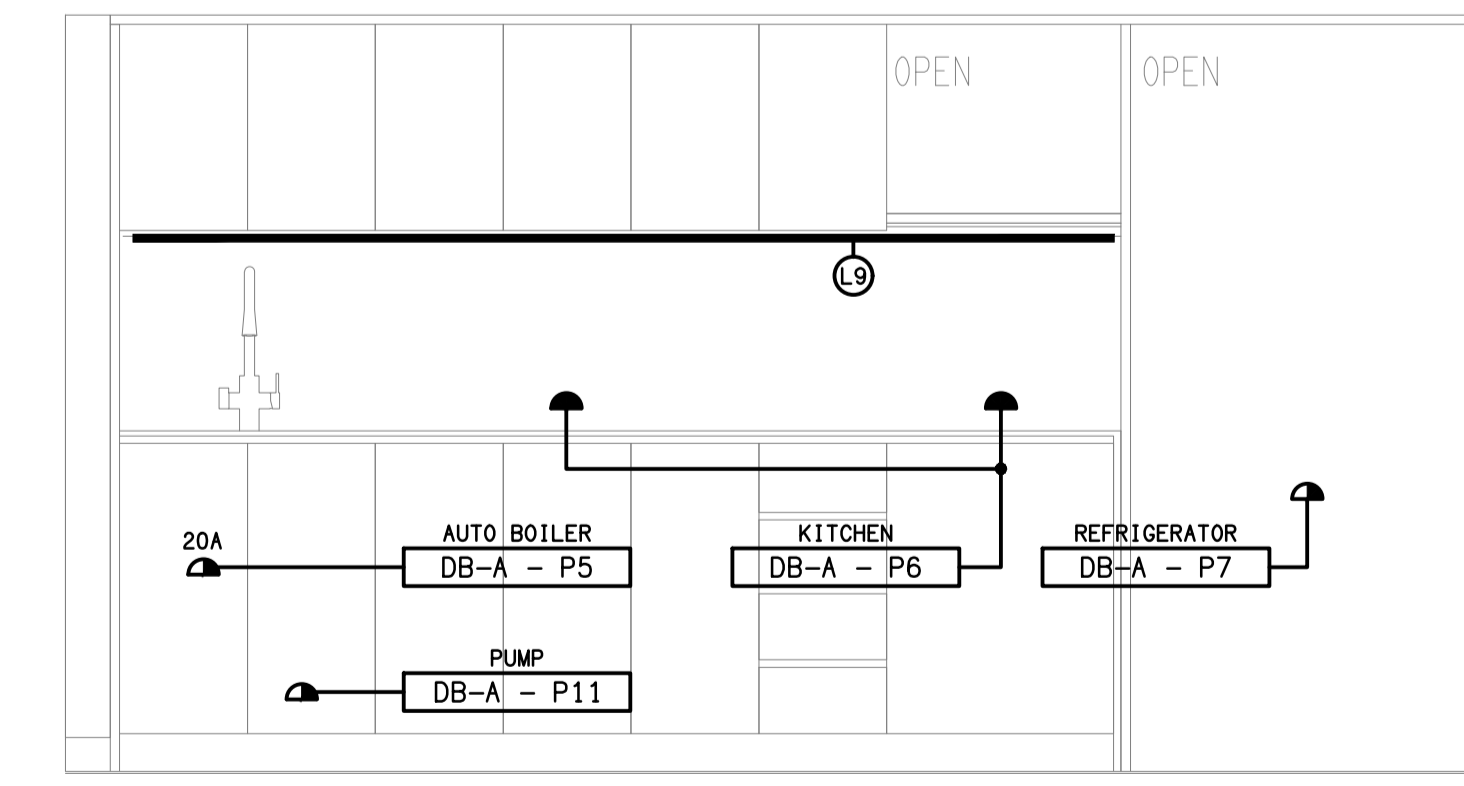
DETAIL A KITCHENETTE ELEVATION SCALE 1:20
